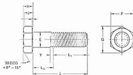
DIMENSION OF HEAVY HEX BOLTS - ANSI/ASME B 18.2.1 in mm
